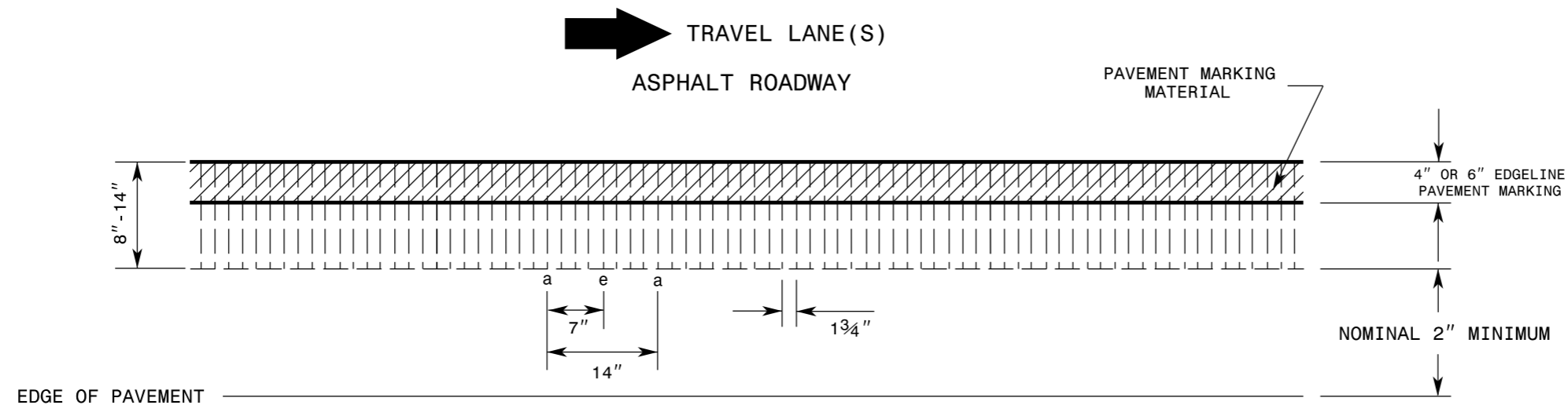
PLAN VIEW
