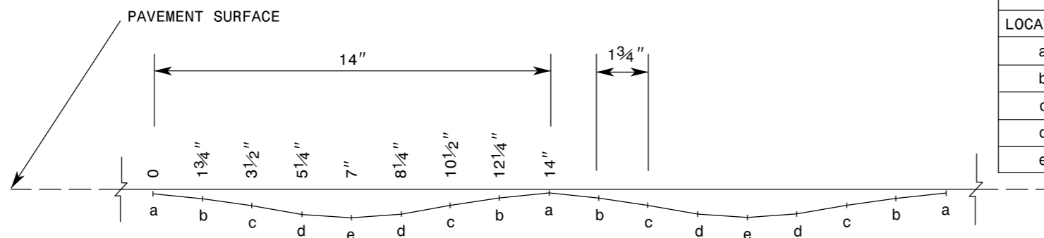
PROFILE VIEW
